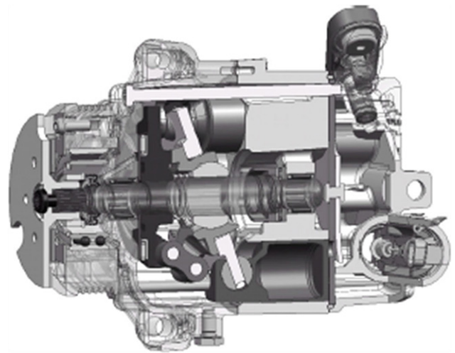
Figure 2 – Pneumatic variable displacement compressor
